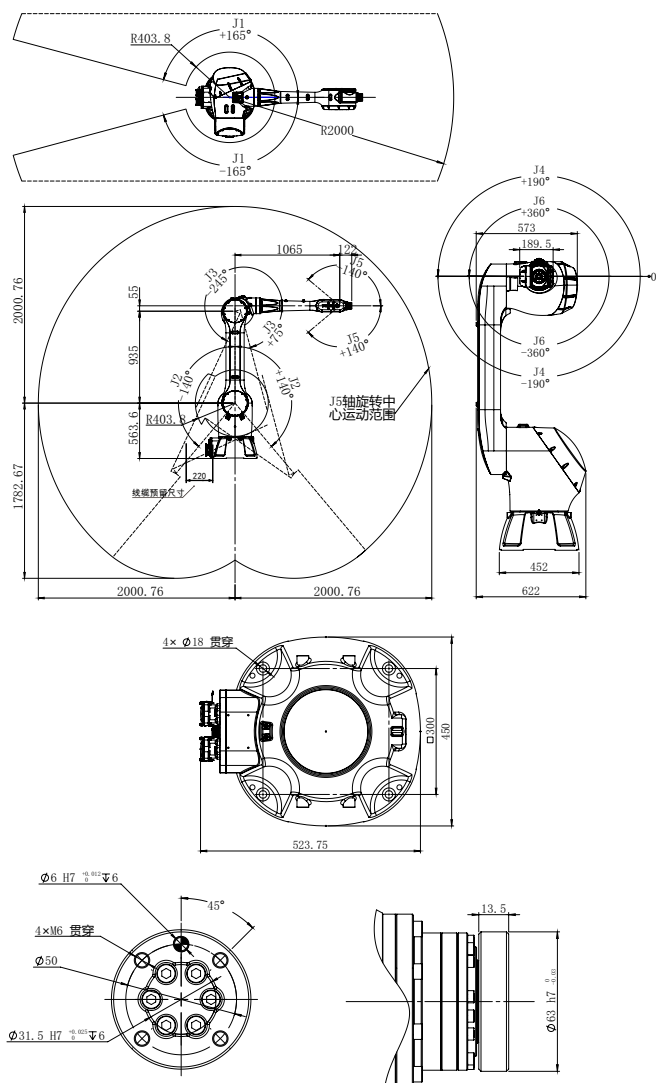
运动空间及外形安装尺寸图 Motion range and installation dimension drawing
