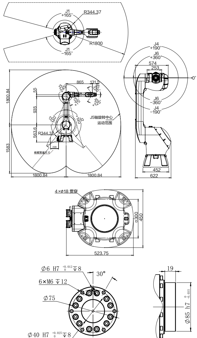
运动空间及外形安装尺寸图 Motion range and installation dimension drawing
