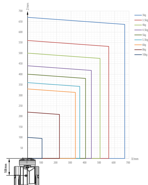
运动空间及外形安装尺寸图 Motion range and installation dimension drawing
