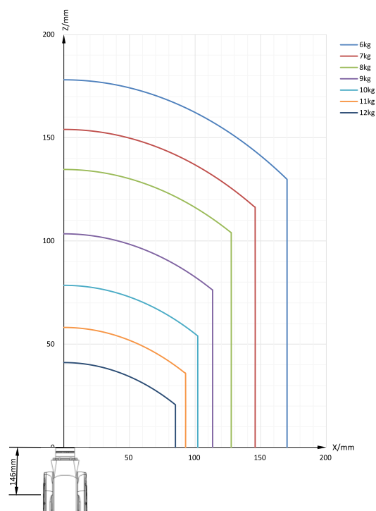
运动空间及外形安装尺寸图 Motion range and installation dimension drawing
