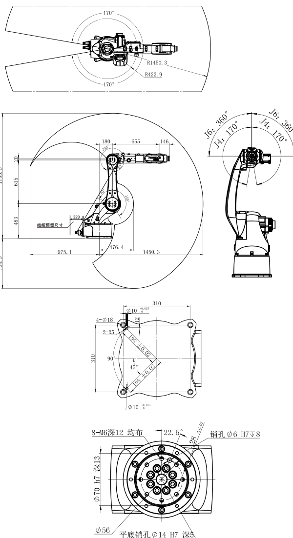
运动空间及外形安装尺寸图 Motion range and installation dimension drawing
