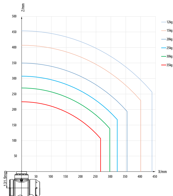
运动空间及外形安装尺寸图 Motion range and installation dimension drawing
